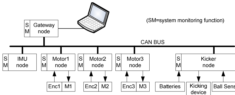
Figure 1. The CAMBADA low-level hardware architecture.
