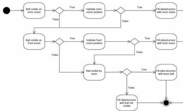
Fig. 12. Ball integration activity diagram.
